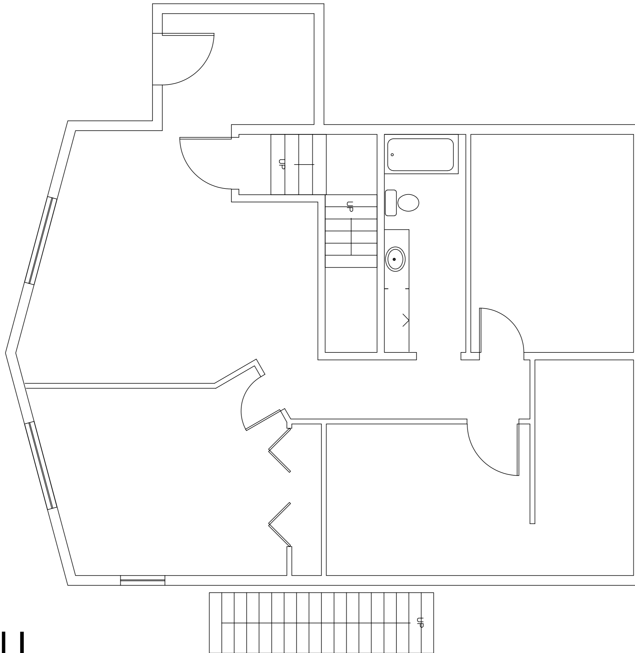
Basement Floor Plan 3/16" = 1'-0"
